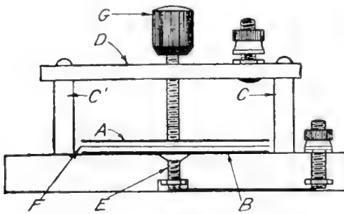
The Distance Between the Plates in This Condenser is Variable
